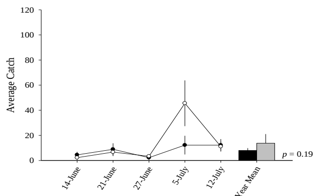
Fig. 1. Averaged catches across all taxa (A & B), Coleoptera (C & D), Lepidoptera (E & F), Orthoptera (G & H), Araneae (I & J), and Hymenoptera: Formicidae (K & L) during 2012 (left column) and 2013 (right column) in pastures which were either rested/deferred or grazed during the early brooding period of late May to early July. Lines represent the average weekly catches, bars represent the averaged catch for the sampling year, and error bars represent the SEM.
