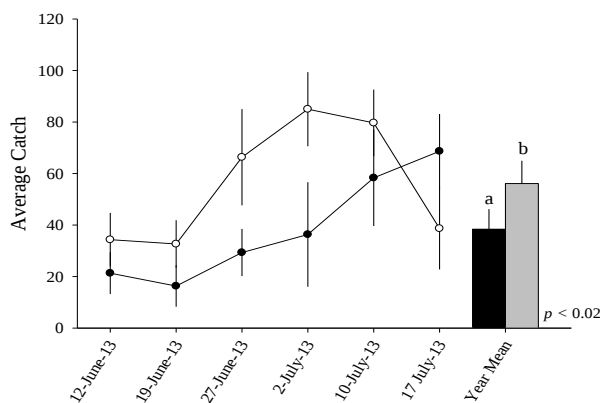
Fig. 1. Averaged catches across all taxa (A & B), Coleoptera (C & D), Lepidoptera (E & F), Orthoptera (G & H), Araneae (I & J), and Hymenoptera: Formicidae (K & L) during 2012 (left column) and 2013 (right column) in pastures which were either rested/deferred or grazed during the early brooding period of late May to early July. Lines represent the average weekly catches, bars represent the averaged catch for the sampling year, and error bars represent the SEM.
