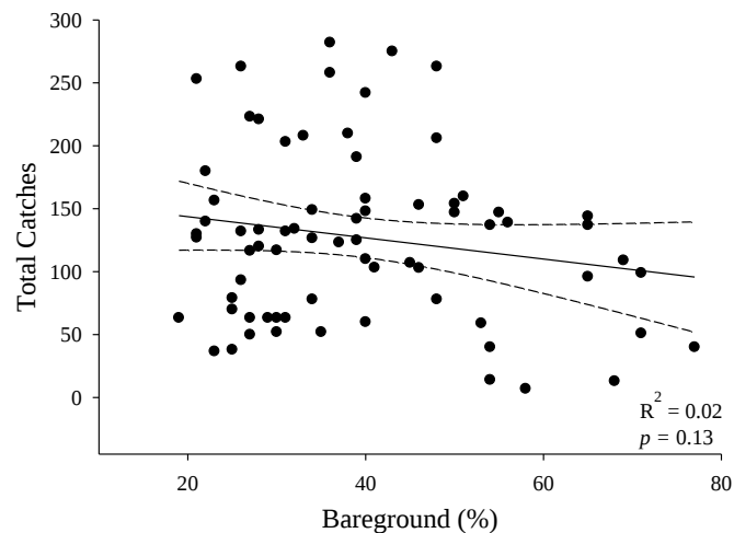
Fig. 3. Linear relationships (solid lines), with 95% confidence intervals (dashed lines), between the total pitfall trap catches across all dates and A) live grass height, B) live sagebrush height, and C) percent bare ground at each of the sampling locations collected from both rested/deferred and livestock grazed pastures. The linear relationships between live grass and sagebrush heights and total arthropods catches are highly significant ( p -value); however the predictive capability ( R^2 ) of each regression equation is low. The linear relationship between the percentage of bare ground and the total seasonal catches is not significant.
