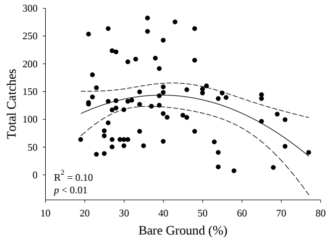
Fig. 2. Polynomial relationships (solid lines), with 95% confidence intervals (dashed lines), between the total pitfall trap catches collected across all dates and A) live grass height, B) live sagebrush height, and C) percent bare ground from sampling locations located in rested/deferred and livestock grazed pastures. The relationship of each regression is highly significant ( p -value); however the predictive capability ( R^2 ) of each equation is low.
