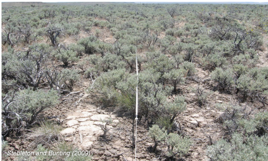
Figure 3. Composition and fuel loading values of a Wyoming big sagebrush steppe in northern Nevada. Low herbaceous fuel loading and high levels of bare ground reduce the probability of fire under low intensity burning conditions.
